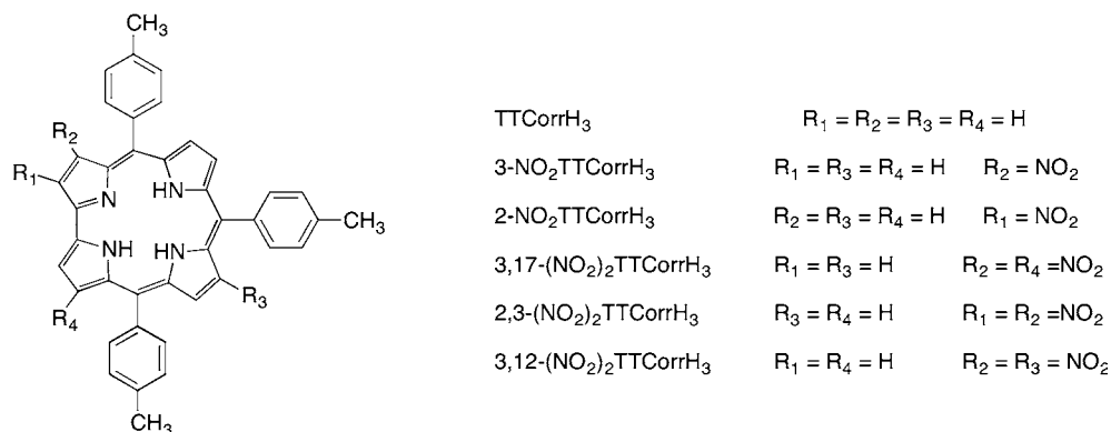
Chart 1. Molecular Structures of \beta -Nitrocorroles Presented in This Work
