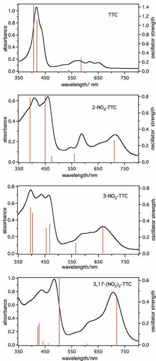
Figure 9. Comparison between computed (TDDFT/B3LYP) and experimental absorption spectra of TTCorrH 3 and its nitro derivatives in CH 2 Cl 2 .
